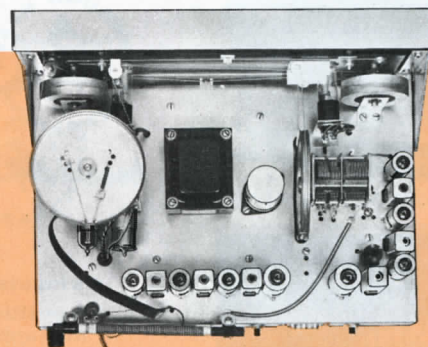
This interior view of the AJ-11 shows the well-planned layout and husky components of this instrument. The circuitry is carefully engineered to assure you easy construction with the best possible results.
