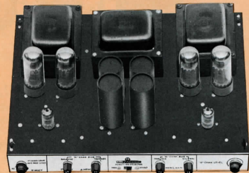
This interior view of the AA-121 Stereo Amplifier shows the rugged, conservatively rated components that can loaf along at full 80 watts output.
