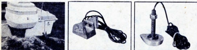
Transom-mount transducer (left) is recommended for high-speed craft with planing hulls. Through-hull transducer (right) is ideal for permanent installation in larger boats with displacement hulls.
