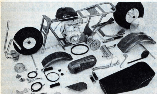
Kit supplied with engine mounted to frame.
