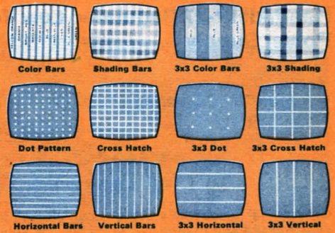
Standard 9x9 display, or exclusive Heath 3x3 display. Produces 12 patterns, plus a clear raster for purity adjustment.
