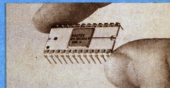
Reliable MOSTEK MOS/LSI integrated circuit "chip", is the "brain" of the GC-1005.
